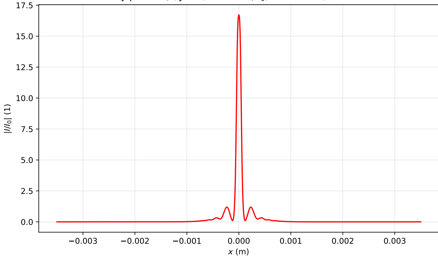
Intensity profile I(x, y = 0, z = 0.478)/I_0 , P_{in}=6.5P_{cr} , artificial time
